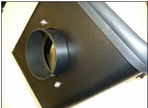
9. Install the filter adapter into the heat shield as shown using the provided hardware.
