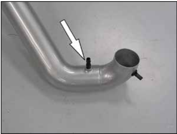
21. Install the provided vent fitting into the K&N® intake tube as shown. NOTE: Plastic NPT fittings are easy to cross thread. Install the vent fitting "hand" tight, then turn it two complete turns with a wrench.
